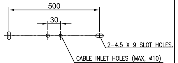
SETTING DIMENSION
